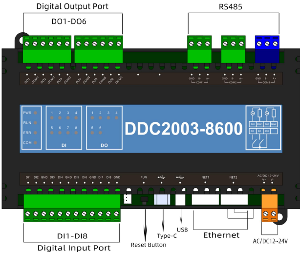
Figure1 Power and Communication Diagram
