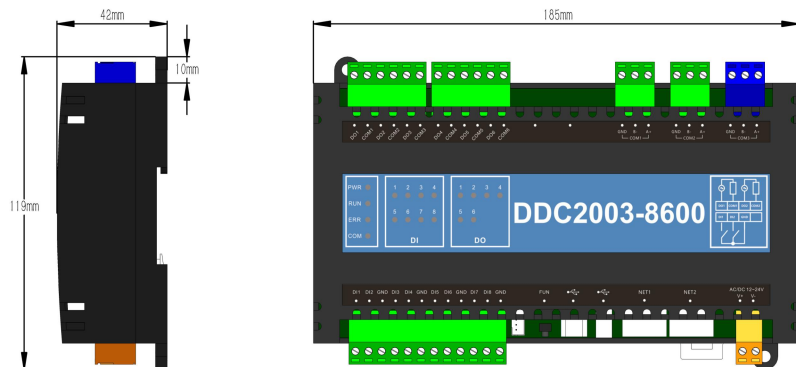
Figure 5 185mm*119mm*42mm(L×W×H) Weight :350g
